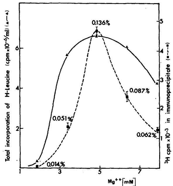
Fig.3. Dependence of TAT synthesis on \text{Mg}^{2+} concentration. Total protein synthesis ( \Delta — \Delta ) was measured by the amount of [ ^3\text{H} ]leucine incorporated. Specific synthesis of TAT ( \blacksquare — \blacksquare ) was measured by immunoprecipitation and is expressed as % total protein synthesis for each given \text{Mg}^{2+} concentration (mean value of 3 different determinations).
