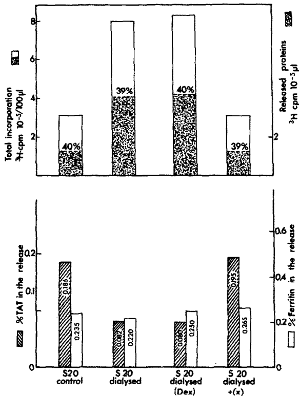
Fig.2. Influence of dialysis of the 'S-20' 20 000 X g supernatant extract. The extracts from dexamethasone-induced cells were dialyzed twice for 30 min (Visking tubing 18/32) against buffer A in the presence or in absence of hormone (Dex) prior incubation with [ ^3\text{H} ]leucine. In the experiment represented in the last column, the concentrated dialysate (X) was added for incubation as described in section 2.
